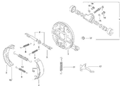
PLATE-39 SET PART Page No. :101-104
